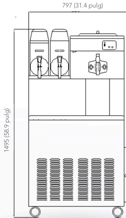
Vista Frontal
